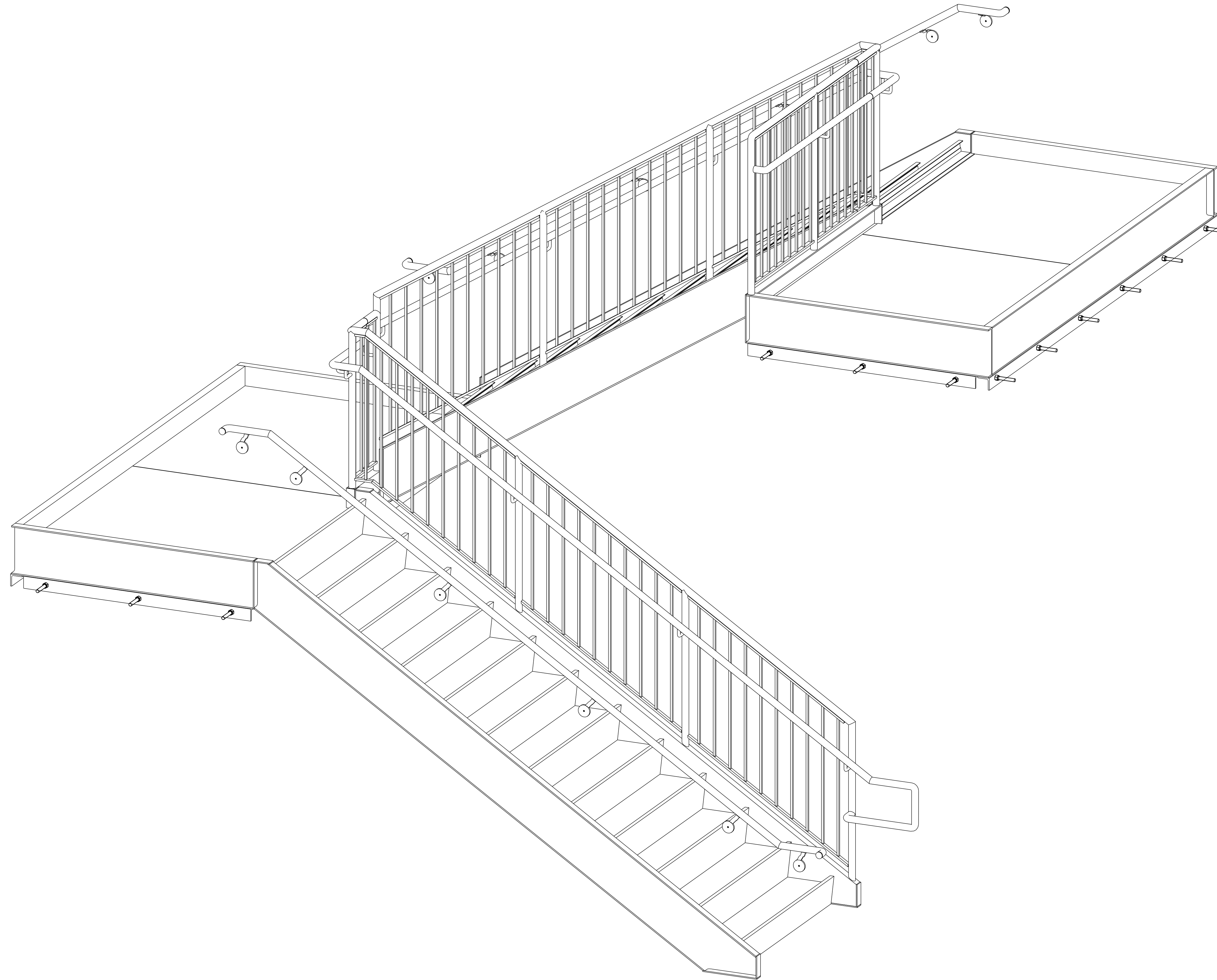
STAIR-A ISOMETRIC VIEW (AREA-A) (REF:A9.1)
