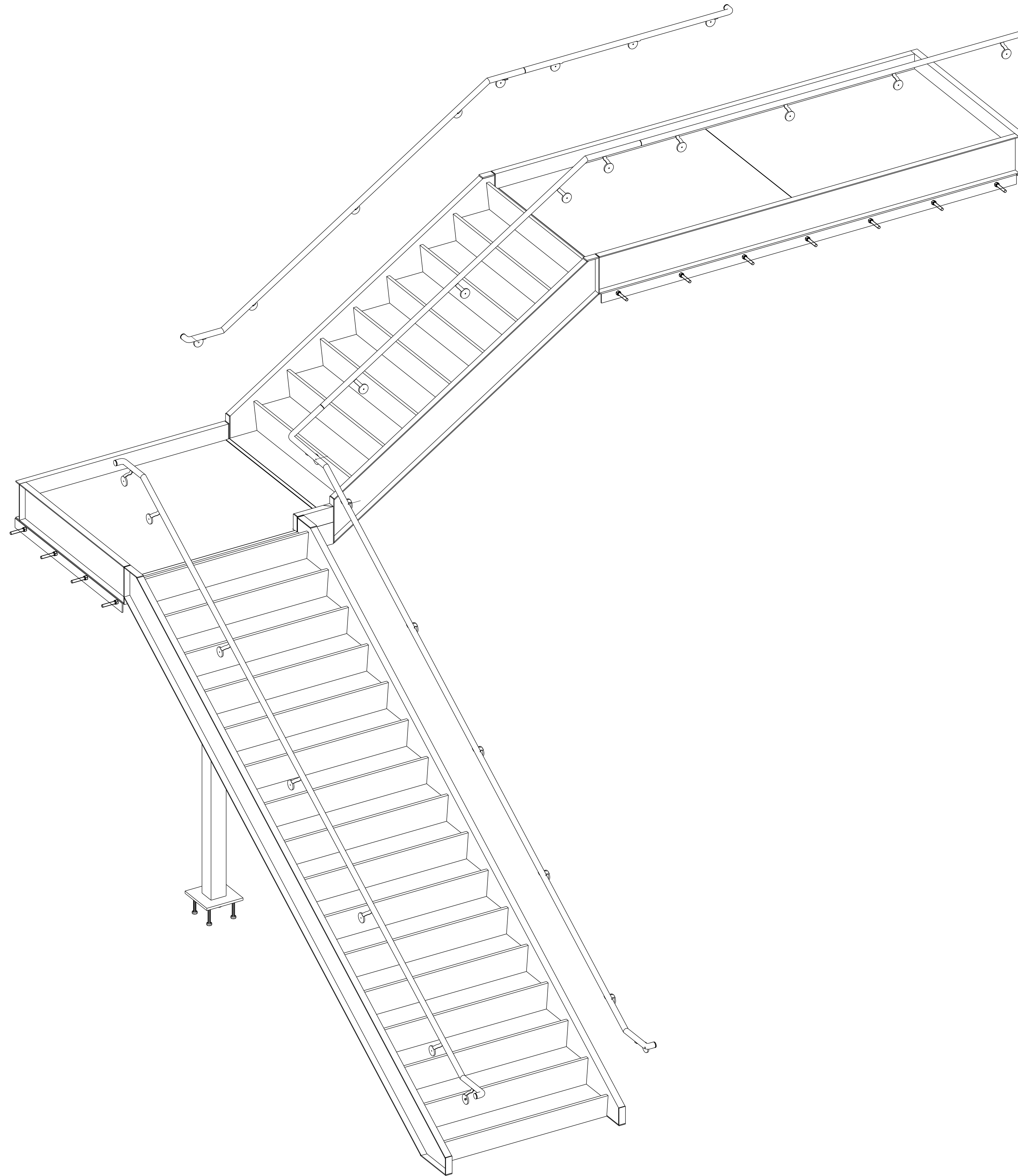
STAIR D-2 ISOMETRIC VIEW (AREA-D.2) (REF DWG:A9.6)
