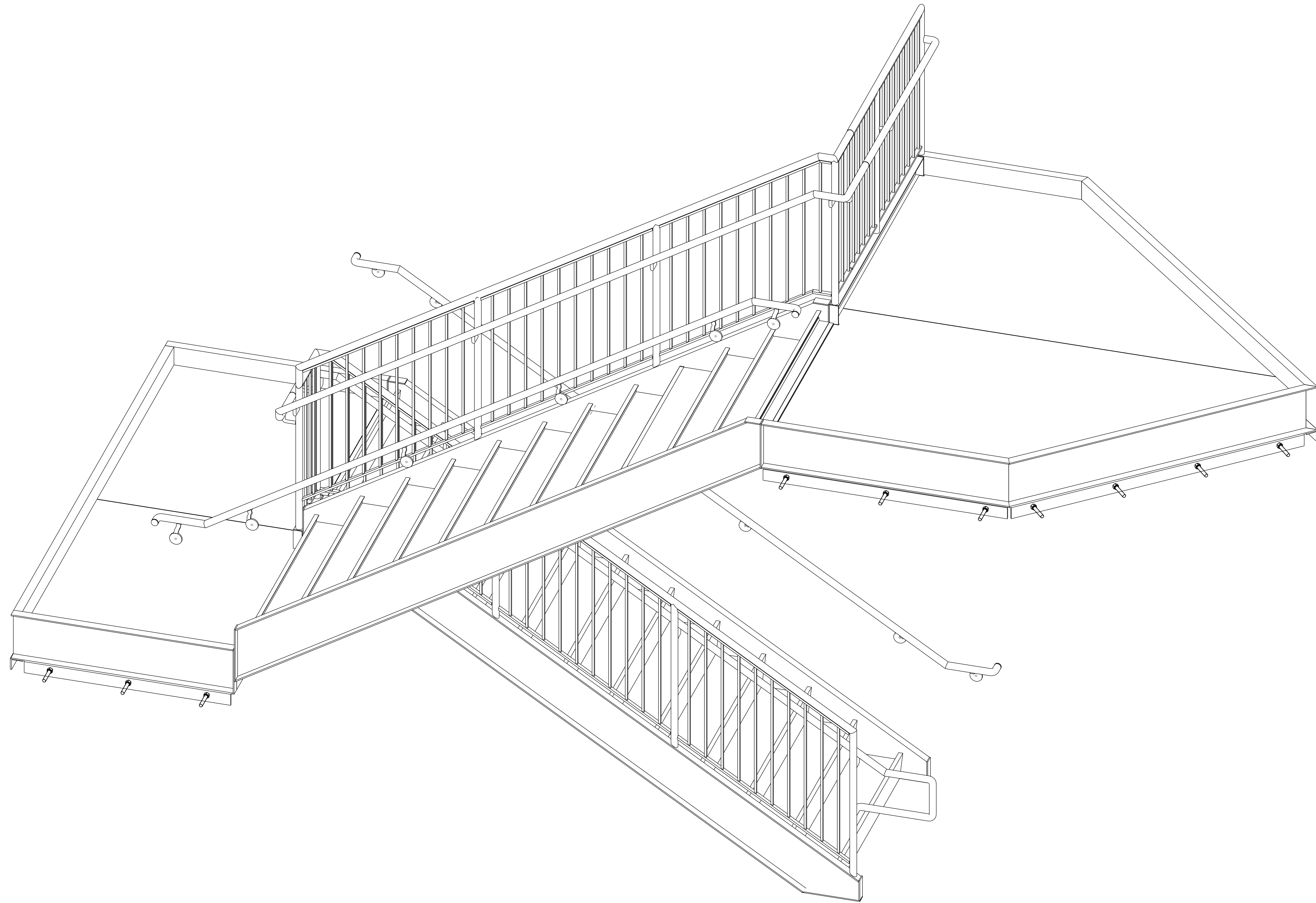
STAIR D-1 ISOMETRIC VIEW (AREA -D.1) (REF DWG-A9.4)
