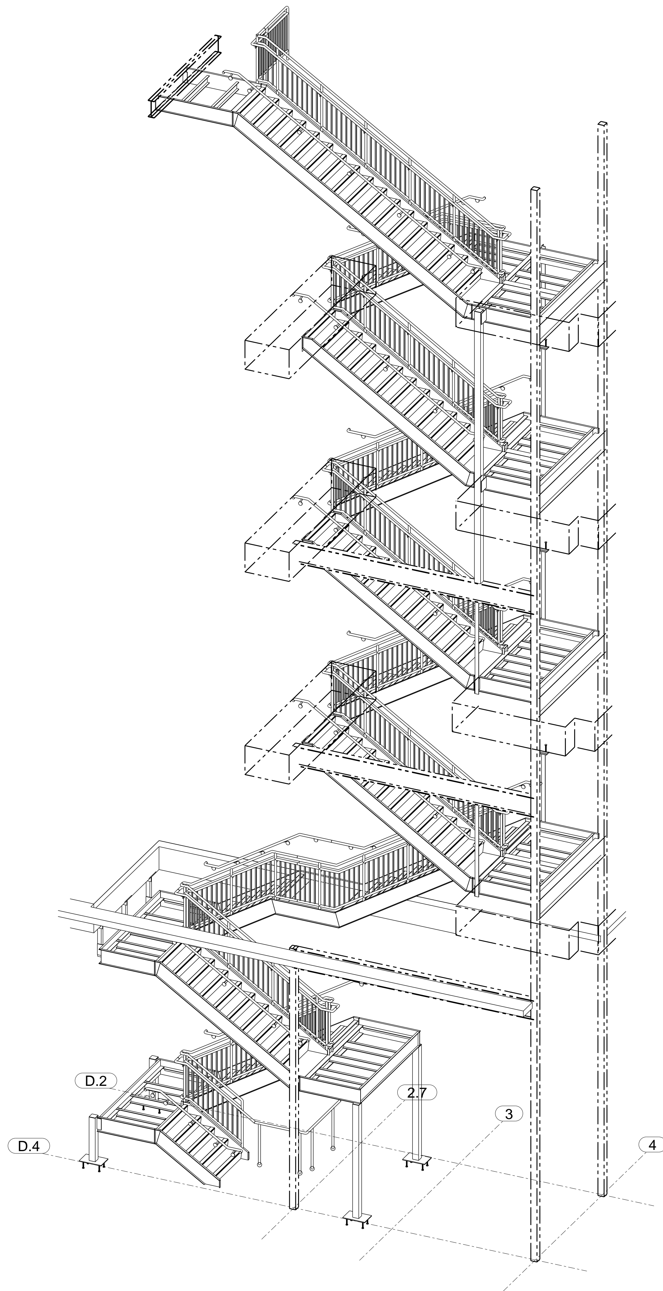
ISOMETRIC VIEW (MAIN BUILDING REF STAIR#101)
