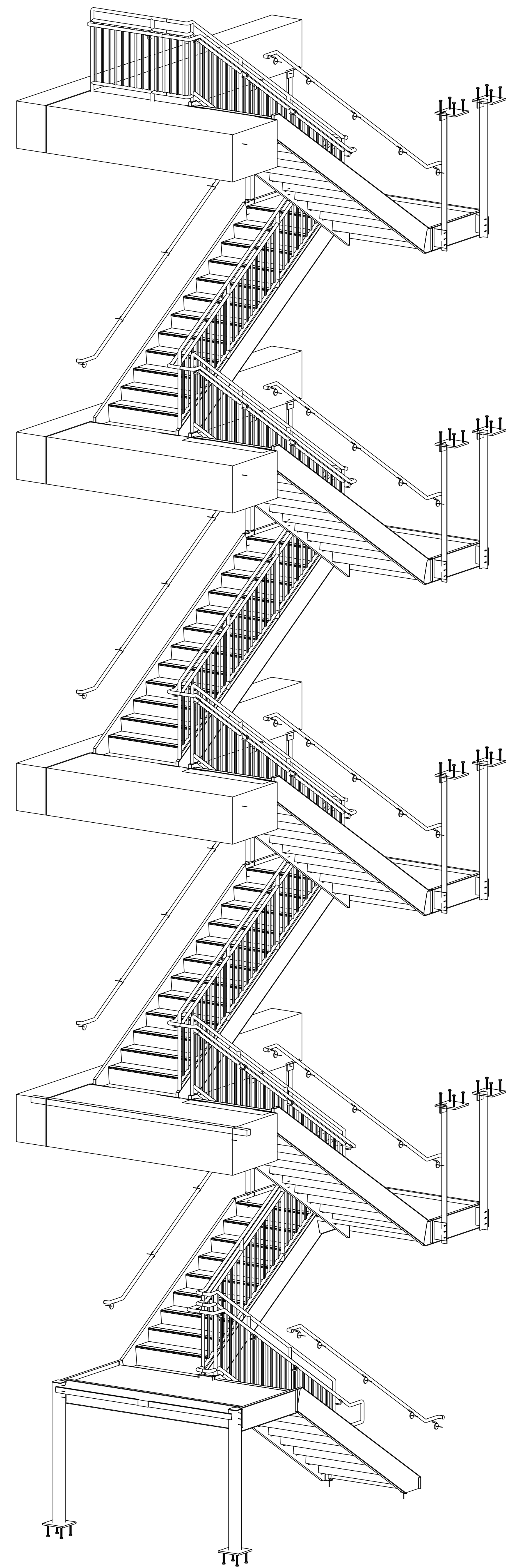
ISOMETRIC VIEW STAIR-107 (MAIN BUILDING)
