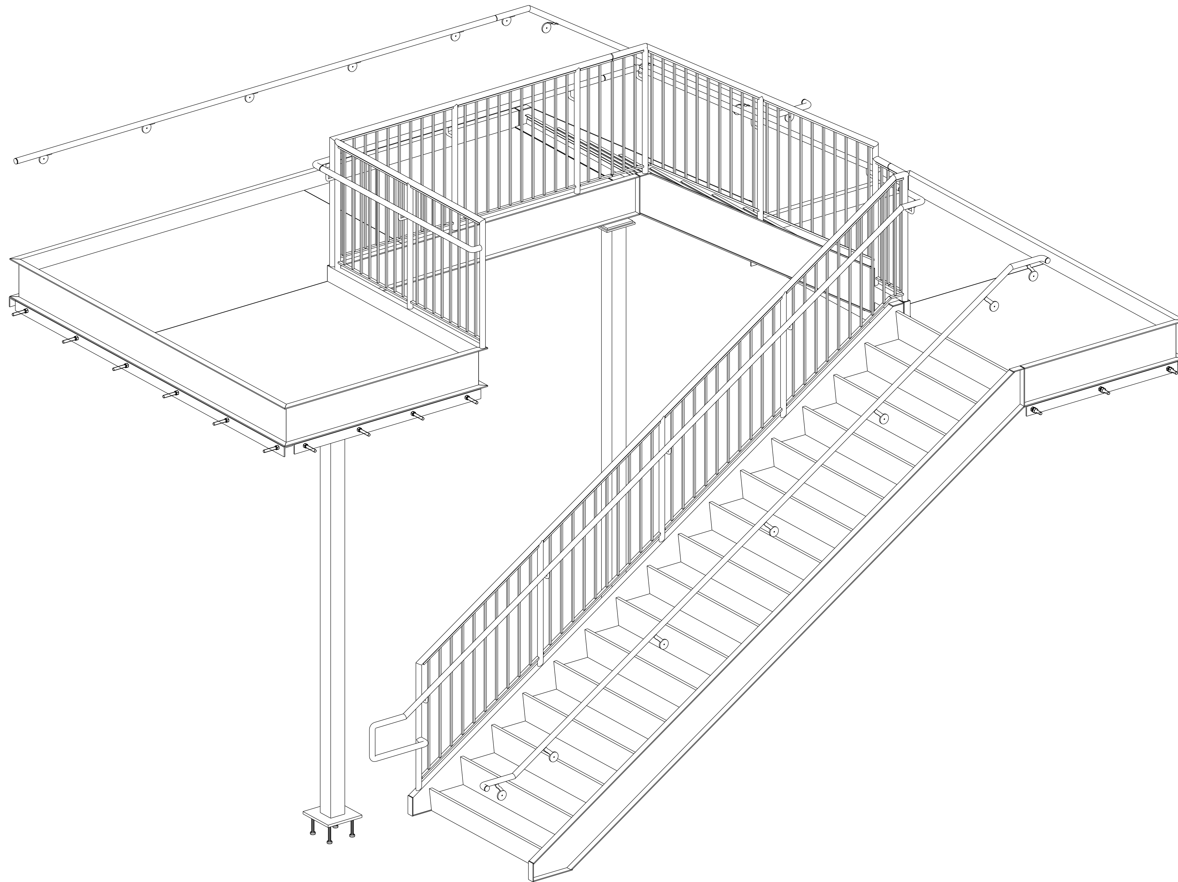
STAIR-C ISOMETRIC VIEW (AREA-C) (REF DWG:A9.3)
