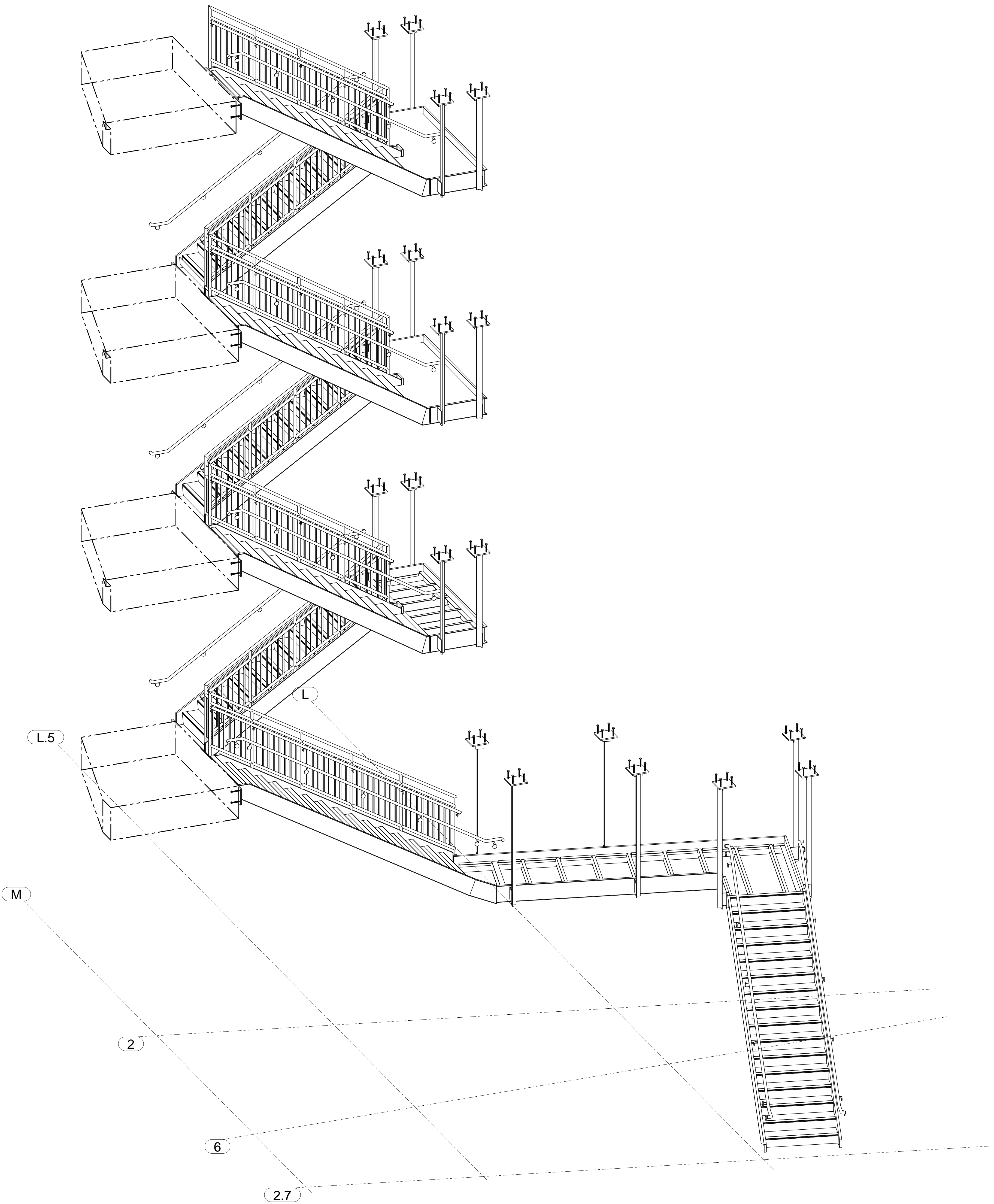
ISOMETRIC VIEW STAIR-102 (MAIN BUILDING)
