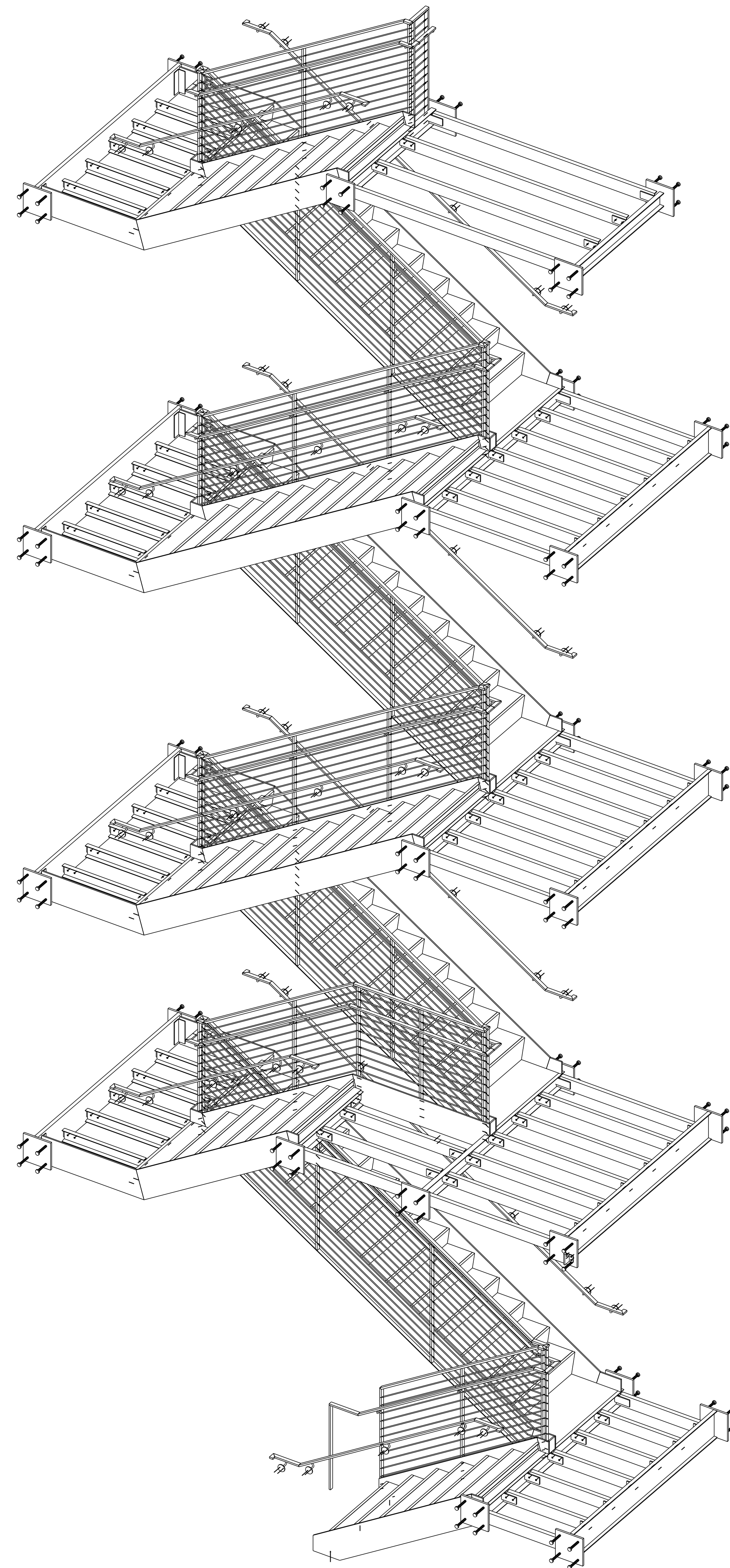
STAIR 2 - ISOMETRIC VIEW (REF:2/A702)
