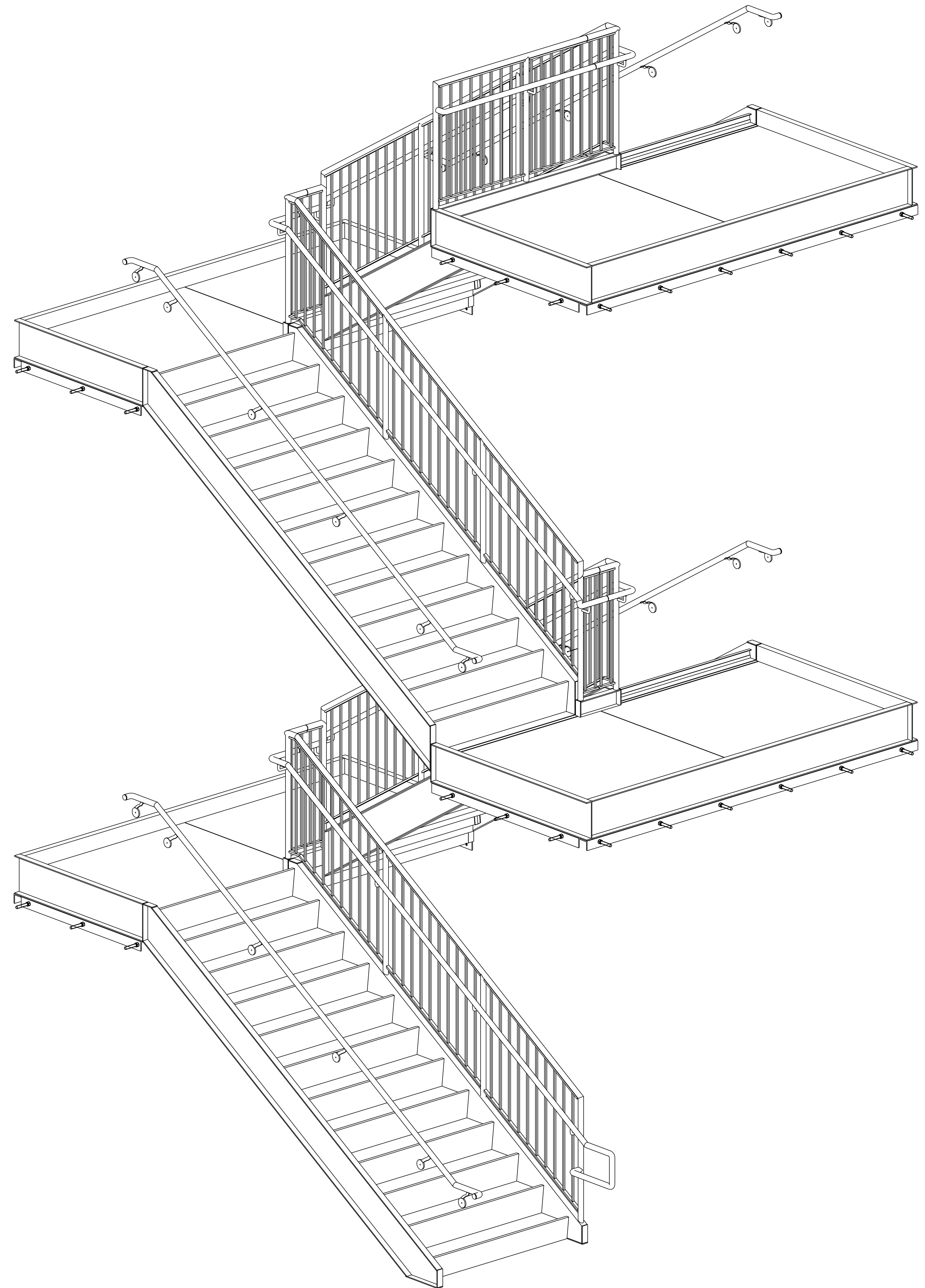
STAIR-B ISOMETRIC VIEW (AREA -B) (REF DWG :A9.2)
