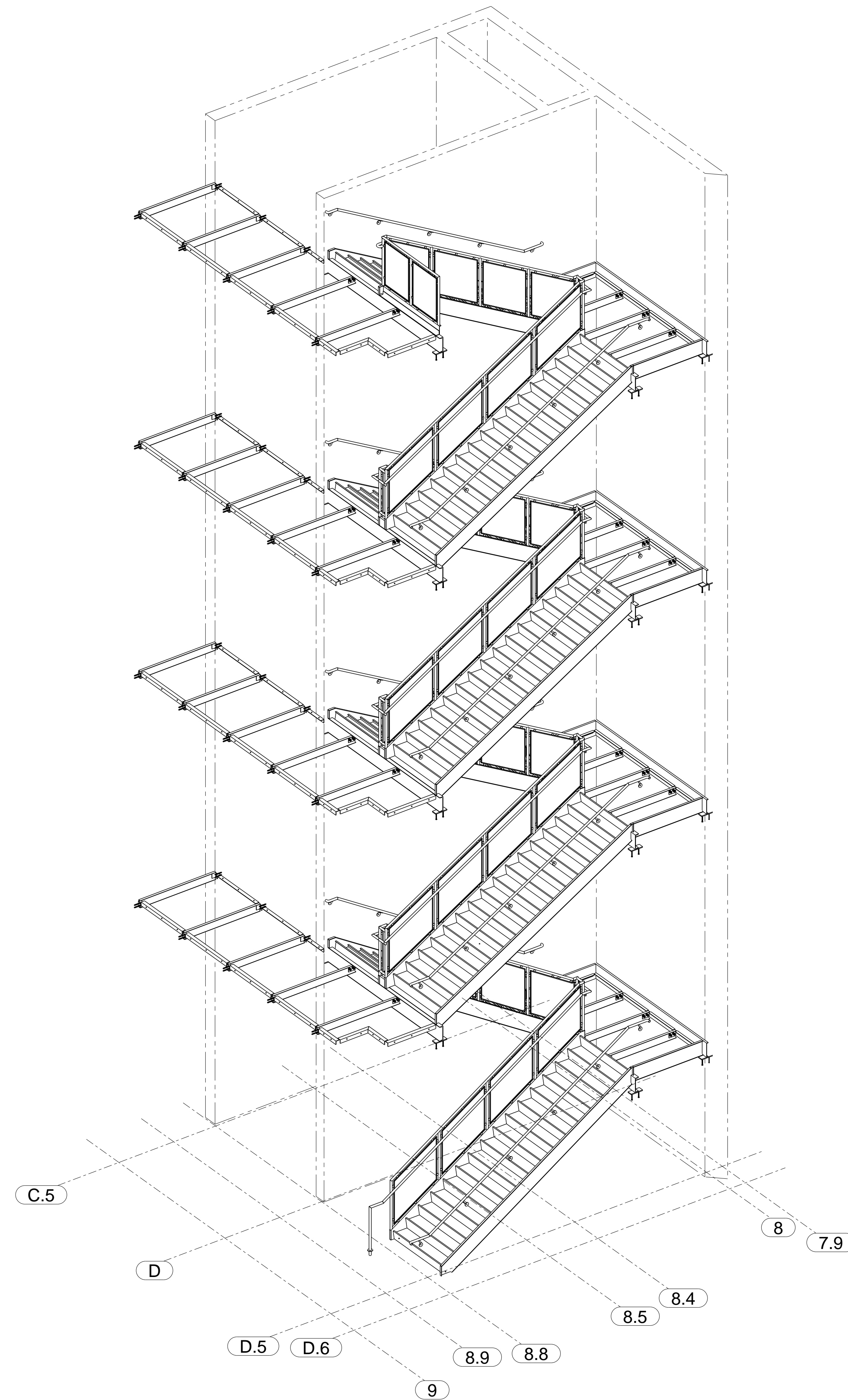
STAIR #1 3D-VIEW
