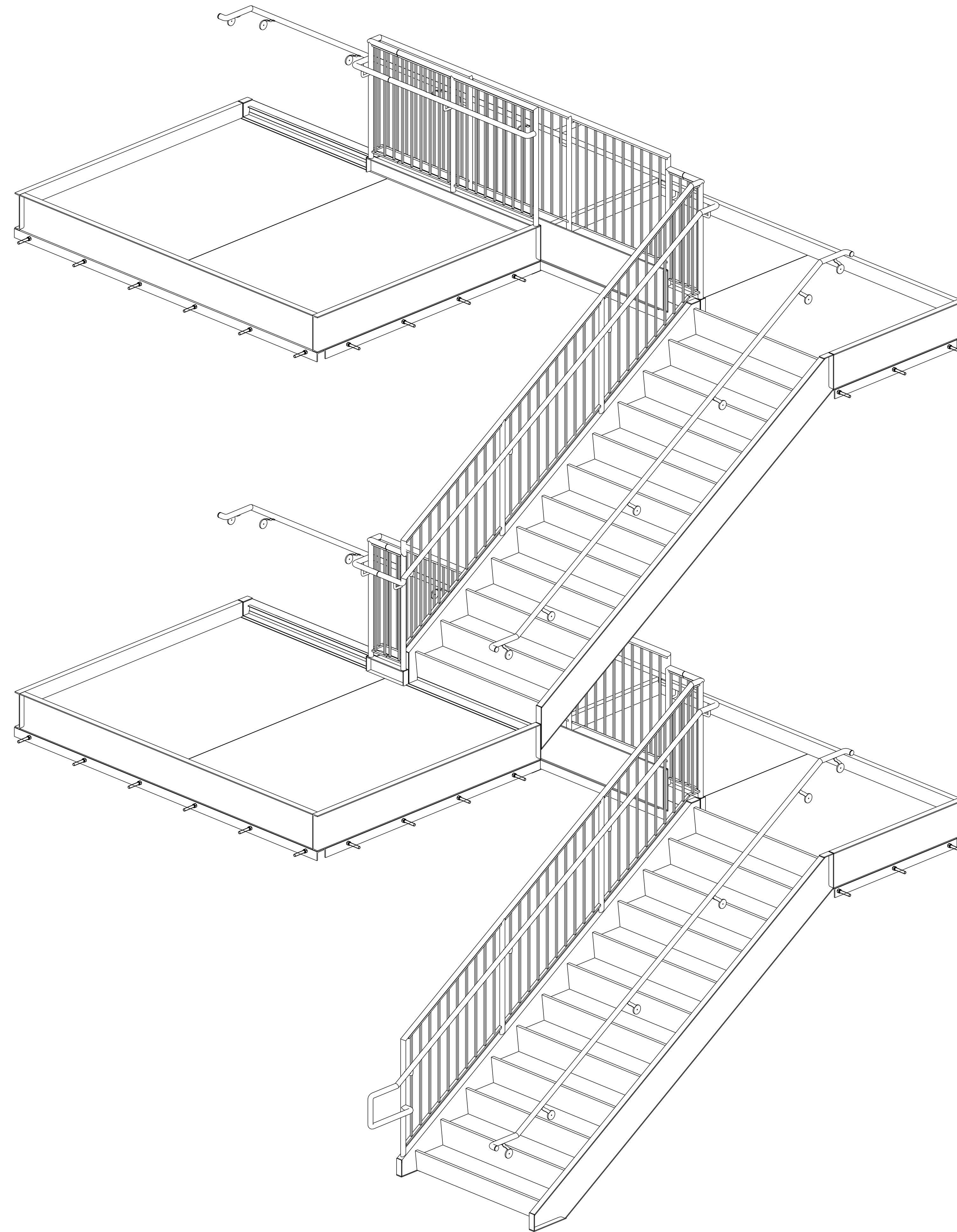
STAIR G ISOMETRIC VIEW (AREA-G) (REF.DWG:A9.7)
