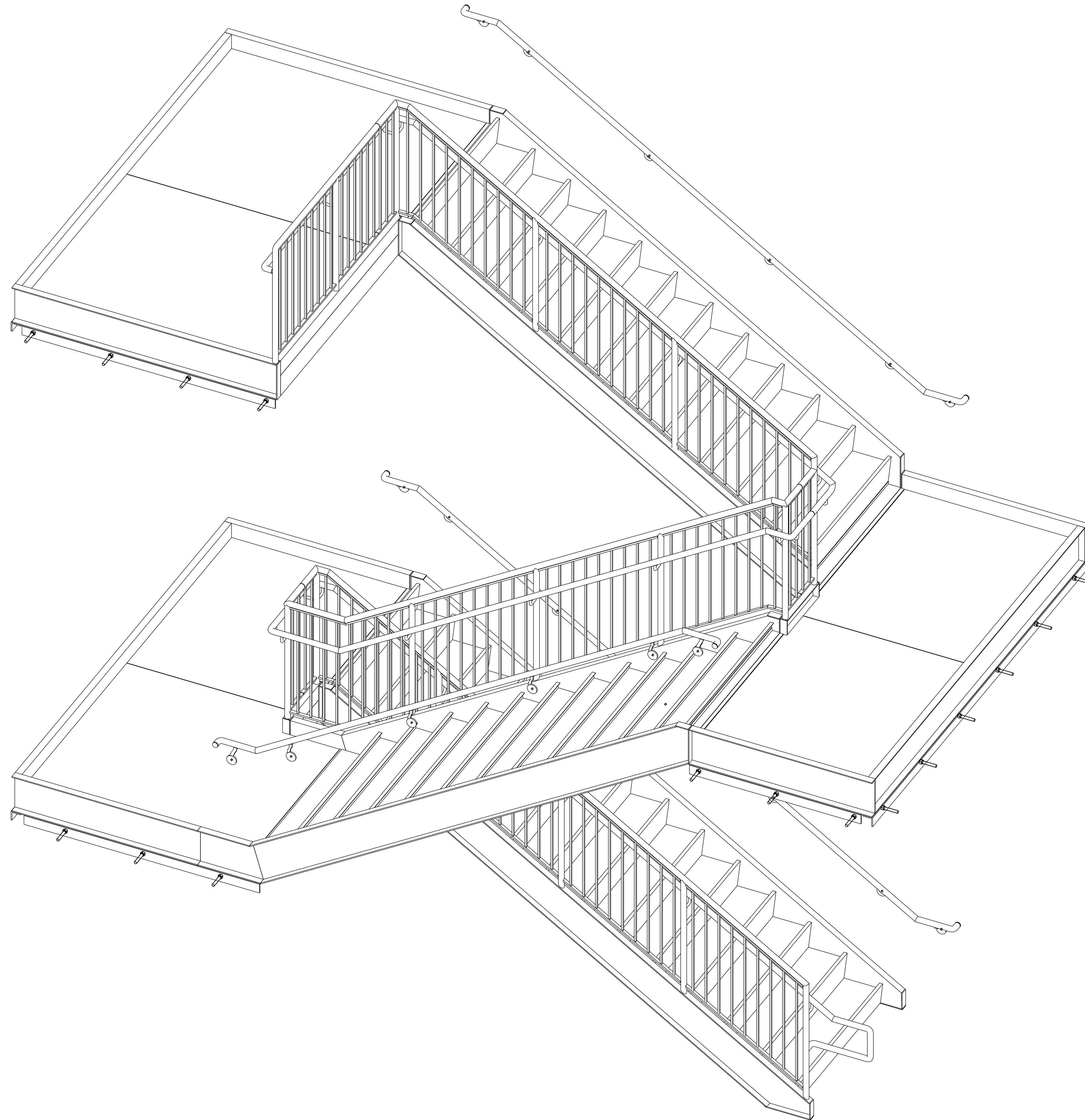
STAIR-H ISOMETRIC VIEW (AREA-H) (REF:A9.8)
